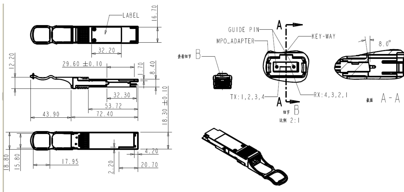
Figure9. Mechanical Specifications
